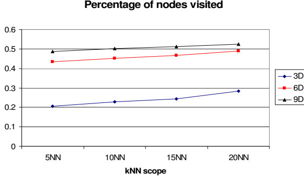
Fig. 12. Effect of k on kNN queries: Percentage of the network nodes that are visited during each range search
