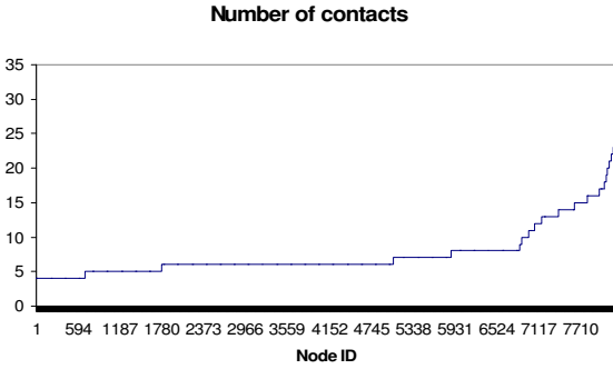
Fig. 5. The number of contact nodes for each node in the network
