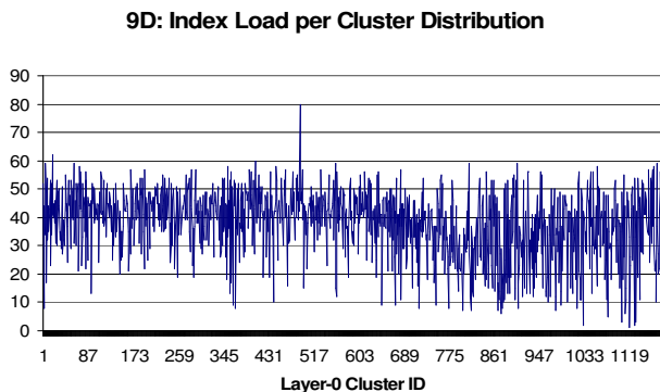
Fig. 9. 9-dimension: The distribution of indices over all layer-0 clusters
