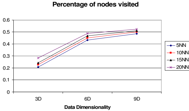
Fig. 13. Effect of dimensionality on kNN queries: Percentage of the network nodes that are visited during each range search
