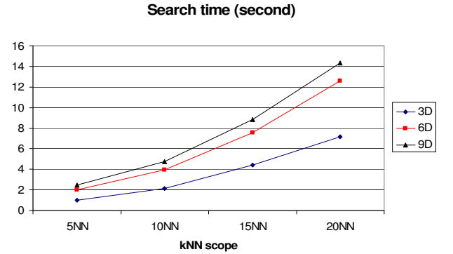
Fig. 15. Effect of k on kNN queries: Search time for each query
