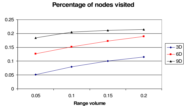
Fig. 10. Effect of volume on range queries: Percentage of the network nodes that are visited during each range search
