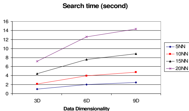
Fig. 17. Effect of dimensionality on kNN queries: Search time for each query
