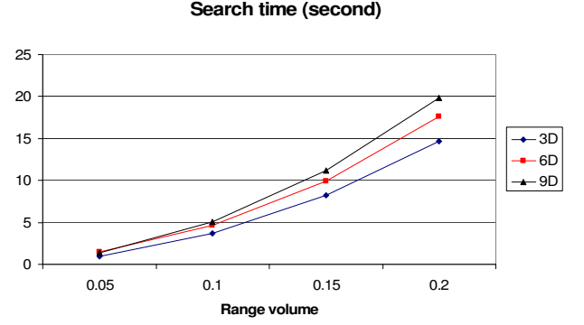
Fig. 14. Effect of volume on range queries: Search time for each query
