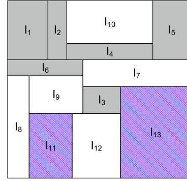
Fig. 3. Examples of index zones in 2-dimension for the hierarchy in Figure 1 and Figure 2: the set of gray rectangles and set of striped rectangles represent the index zones of node 17 and 45, respectively. Each single rectangle represents an index zone at layer 0
