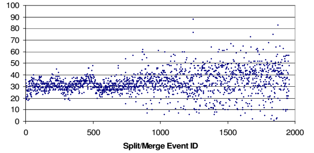
Fig. 7. 9-dimension: Index migration overhead
