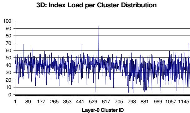
Fig. 8. 3-dimension: The distribution of indices over all layer-0 clusters
