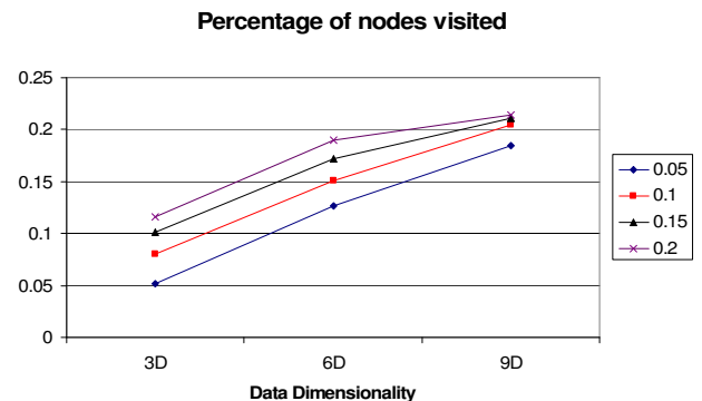
Fig. 11. Effect of dimensionality on range queries: Percentage of the network nodes that are visited during each range search
