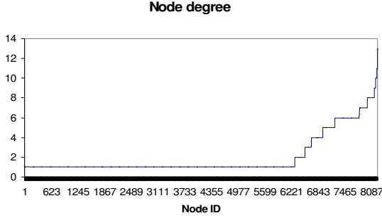
Fig. 4. The node degree for every node in the network
