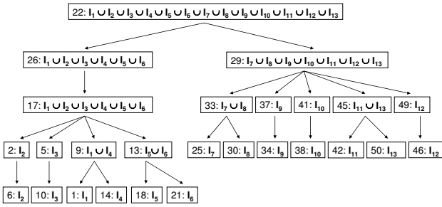
Fig. 2. Index zone assignments of the 52-node Zigzag-4 hierarchy shown in Figure 1
