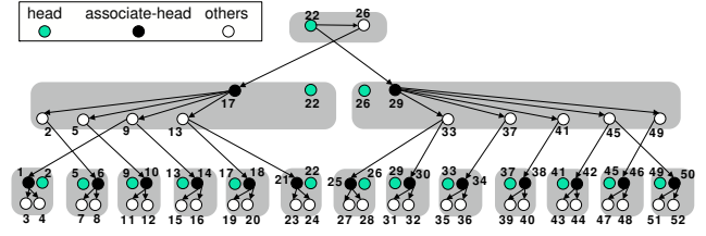
Fig. 1. A zigzag-4 hierarchy of 52 nodes
