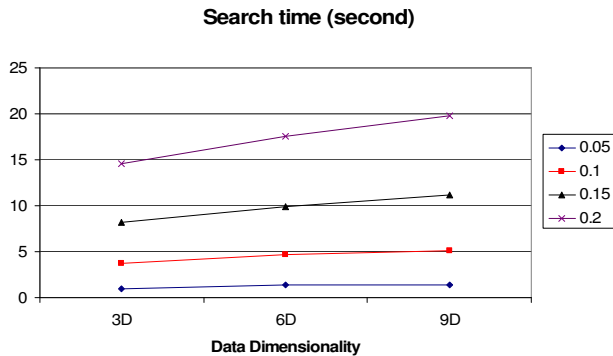
Fig. 16. Effect of dimensionality on range queries: Search time for each query
